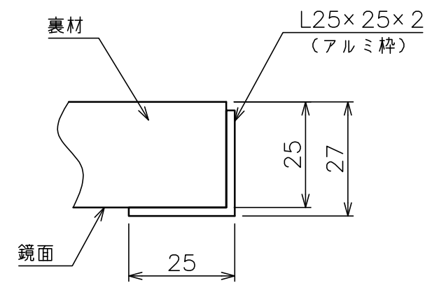
"a"部詳細
