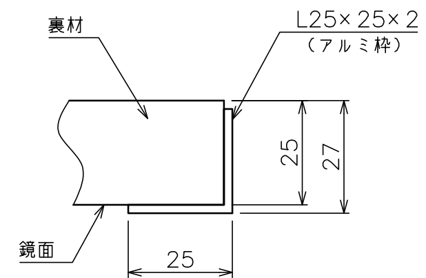
"a"部詳細
