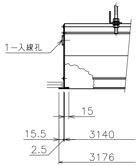
"a"部詳細
