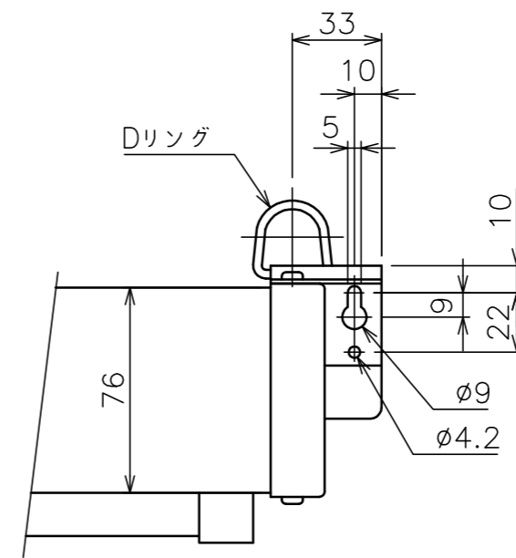
"a"部詳細
