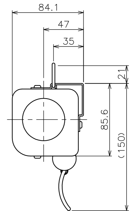
"a"部詳細
