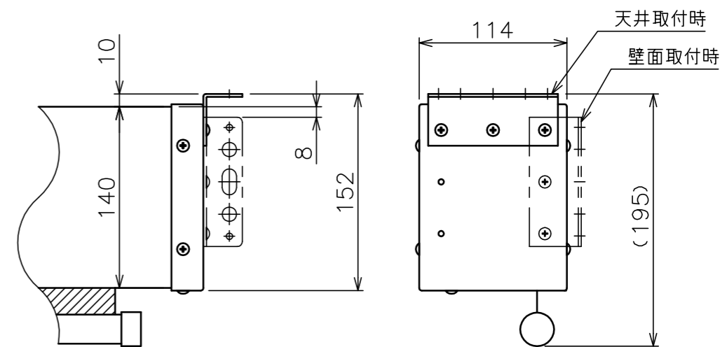
"a"部詳細
