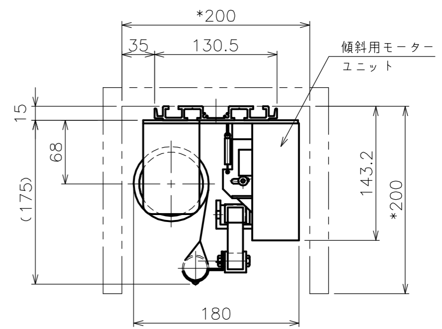
"a"部詳細
